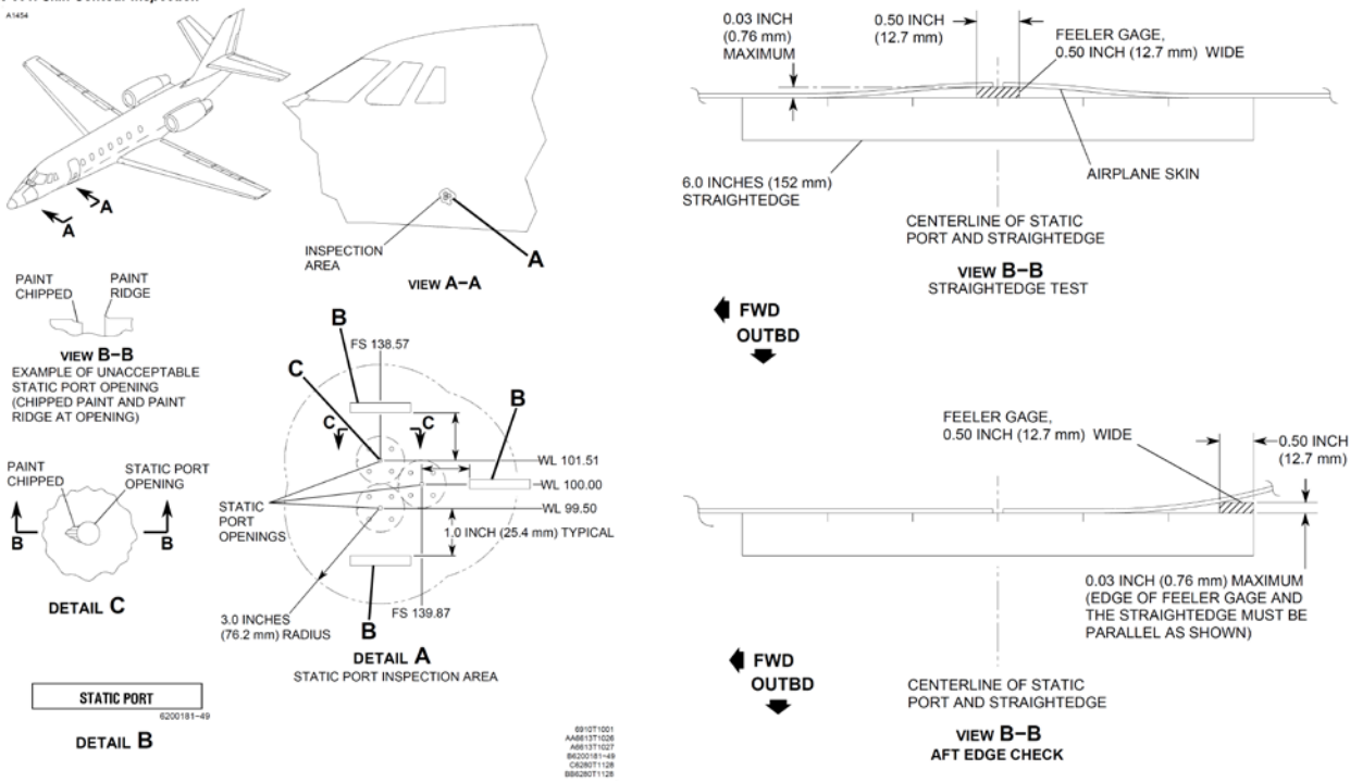
Figure 601. Skin Contour Inspection
